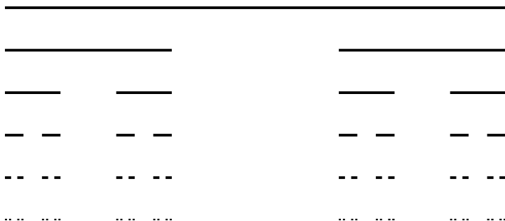
Fig. 5.5. Recursive construction of the Cantor set (top to bottom, omitting each time the middle third of every interval)
