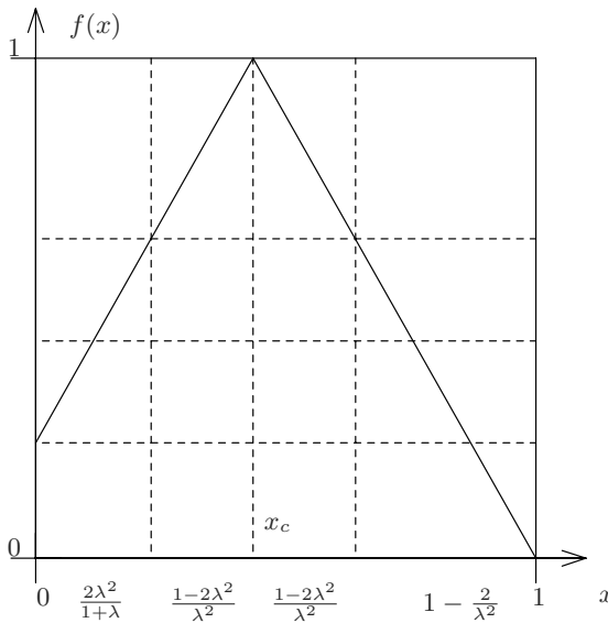
Fig. 9.4. The Baladi map. It is a Markov map
